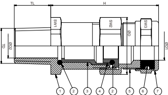
NPT Thread
